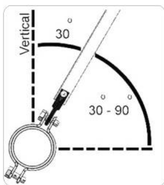
Lateral
