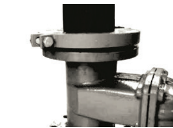
6. Connect mating flange Align flange bolt holes with mating flange (or valve) bolt holes. Insert a standard flange bolt through bolt hole and hand tighten a nut. Insert another bolt opposite the first and hand tighten a nut. Continue this until all bolt holes are fitted. Tighten nuts evenly to specified bolt torque, so flange faces remain parallel. Assembly completed.
