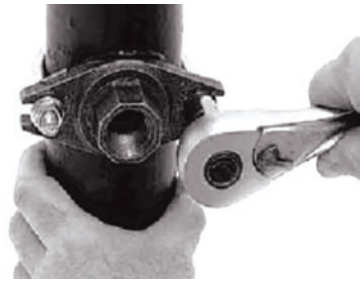
5. Tighten nuts Alternatively and evenly tighten the nuts to the specified bolt torque.
